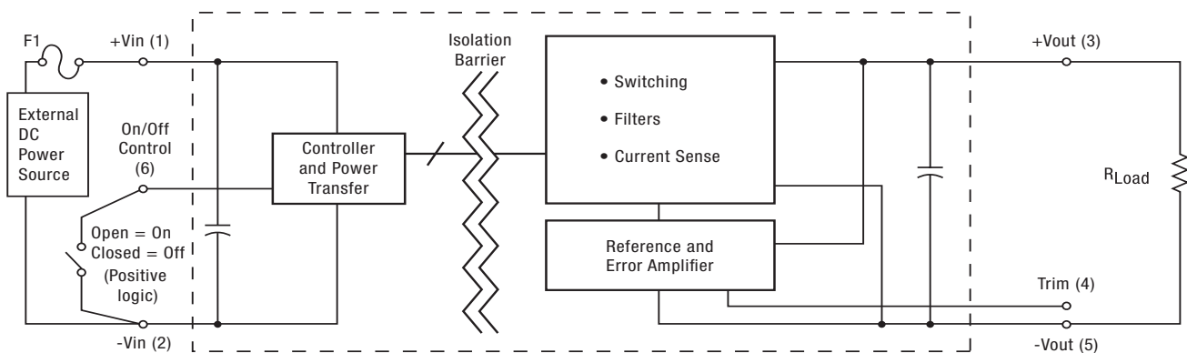
Figure 1. Connection Diagram
