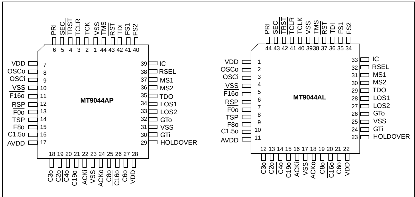
Figure 2 - Pin Connections
