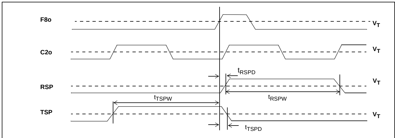
Figure 21 - Output Timing 2
