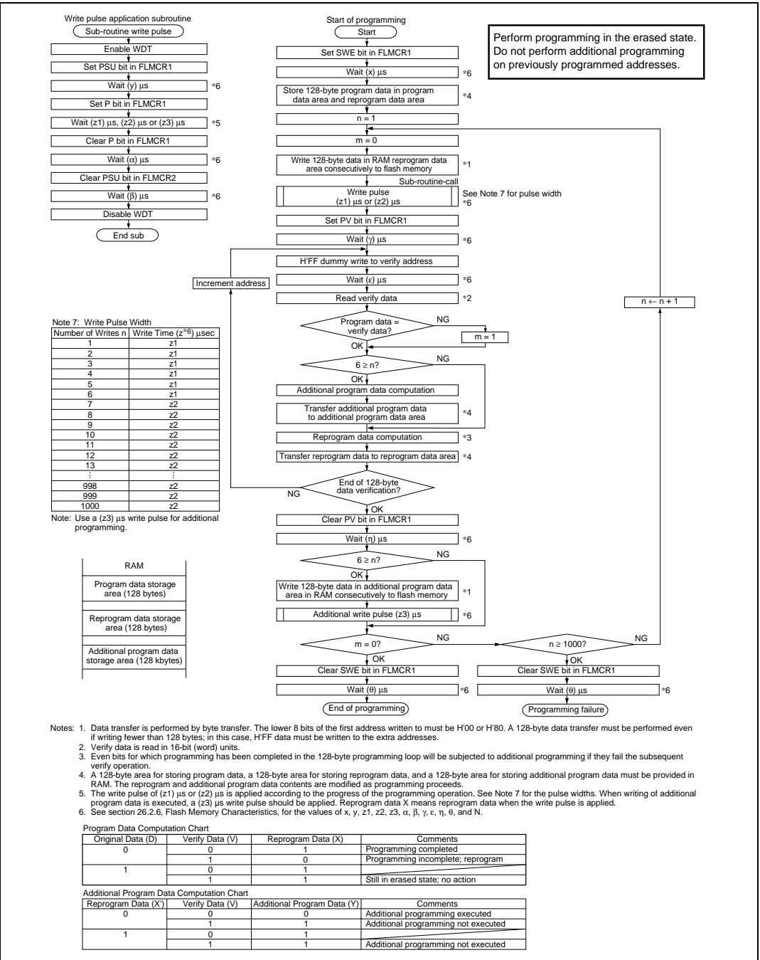
Figure 23.12 Program/Program-Verify Flowchart
