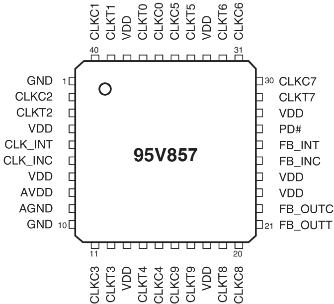
40-Pin MLF
