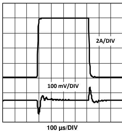
Figure 7-3. V_{IN} = 8\text{ V} , V_{OUT} = 3.3\text{ V} , I_{LOAD} = 2\text{ A} to 10\text{ A} , CH1: V_{OUT} , CH2: I_{LOAD}
