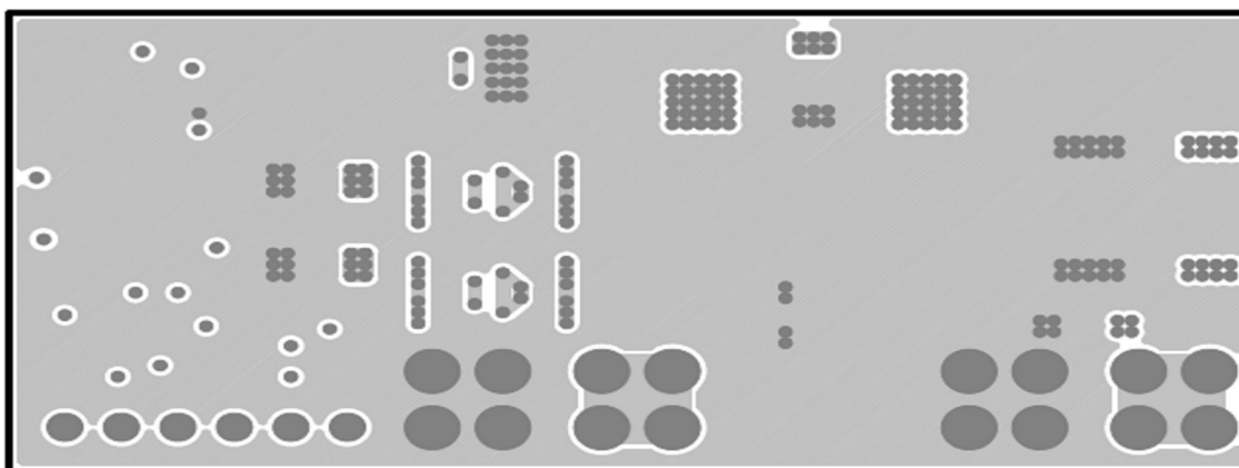
Figure 9-6. Internal Layer-2 (GND Copper)
