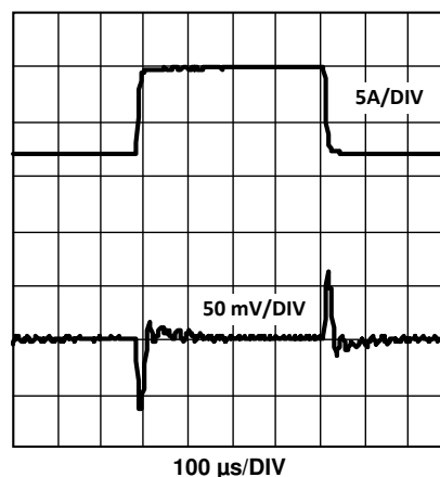
Figure 7-2. V_{IN} = 14\text{ V} , V_{OUT} = 3.3\text{ V} , I_{LOAD} = 11\text{ A} to 19\text{ A} , CH1: V_{OUT} , CH2: I_{LOAD}
