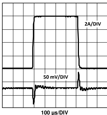
Figure 7-1. V_{IN} = 14\text{ V} , V_{OUT} = 3.3\text{ V} , I_{LOAD} = 2\text{ A} to 10\text{ A} , CH1: V_{OUT} , CH2: I_{LOAD}
