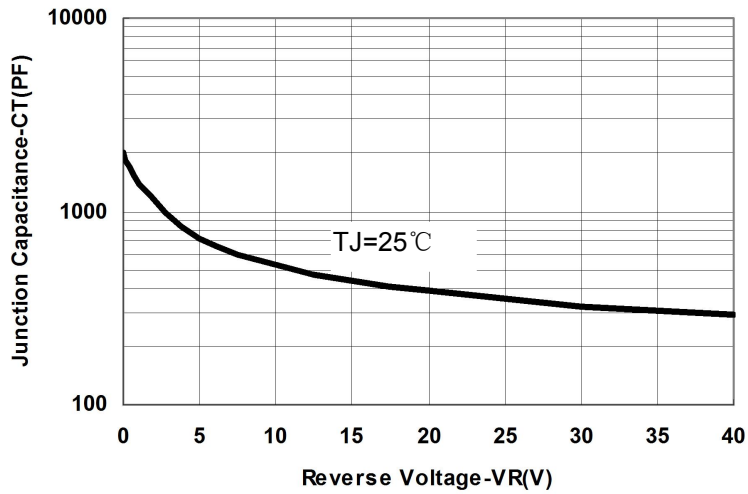
Fig.1-Typical Junction Capacitance
