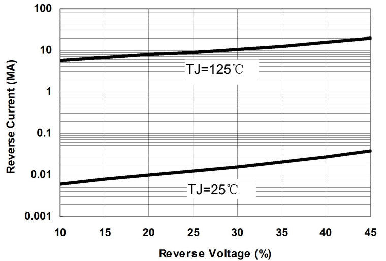
Fig.2-Typical Reverse Characteristics
