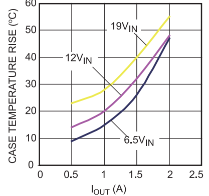
Case Temperature Rise vs. IOUT
