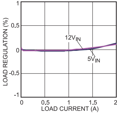
Load Regulation
