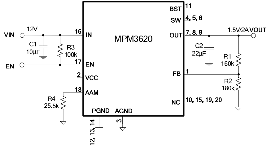
Figure 16. V_{OUT}=1.5V , I_{OUT}=2A
