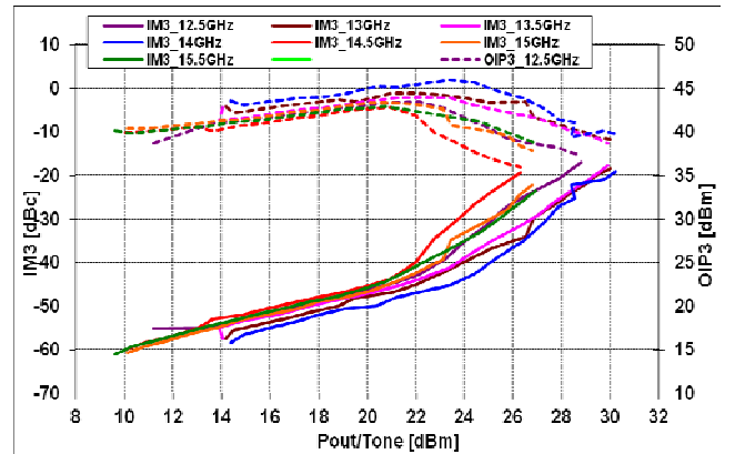
@ V_{ds}=5V, I_{dsq}=2500mA
