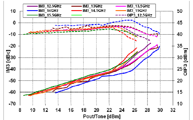
@ V_{ds}=5V, I_{dsq}=2000mA
