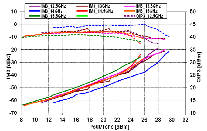
@ V_{ds}=5V, I_{dsq}=1400mA
