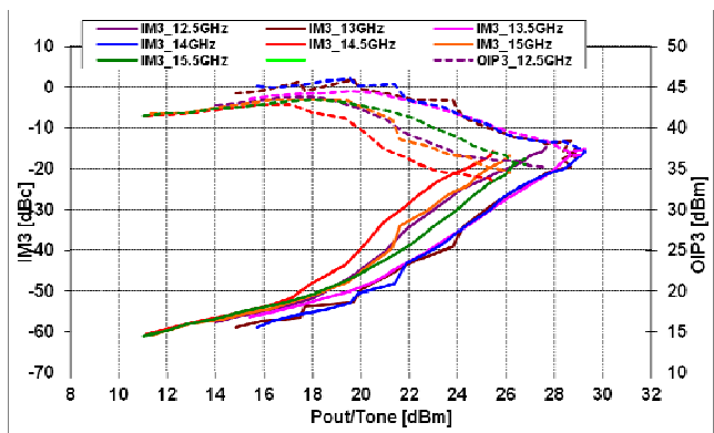
@Vds=4V, Idsq=2500mA
