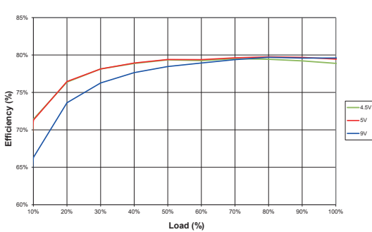
NCM6S0505C
