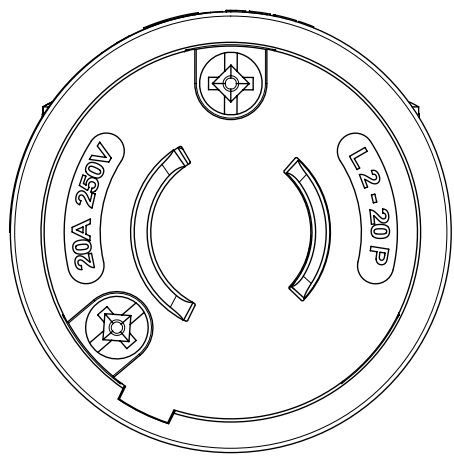
FACE VIEW
