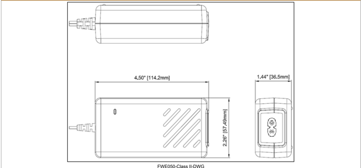
FWE050-Class II-DWG
