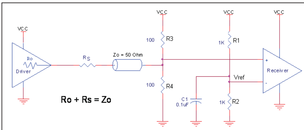
FIGURE 2. SINGLE ENDED SIGNAL DRIVING DIFFERENTIAL INPUT
