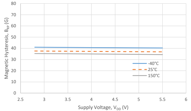
Hysteresis (B) vs. Supply Voltage
