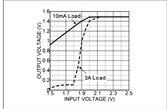
FIGURE 2-5: Dropout Characteristics (1.5V).
