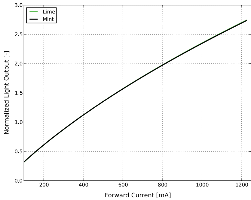
Figure 3d. Typical normalized light output vs. forward current for LUXEON C Mint and Lime at T_j=85^{\circ}\text{C} .
