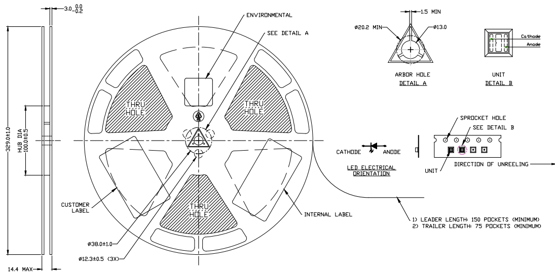
Figure 16. Reel dimensions for LUXEON C Color Line.
