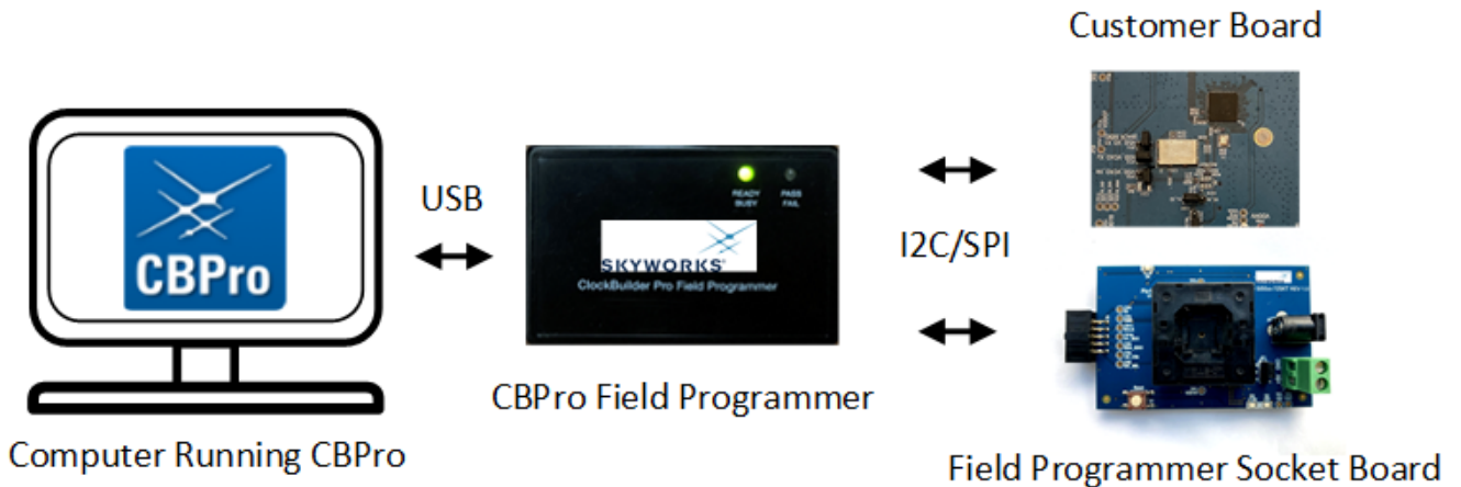
Figure 4.1. PC to CBPROG-DONGLE Connection
