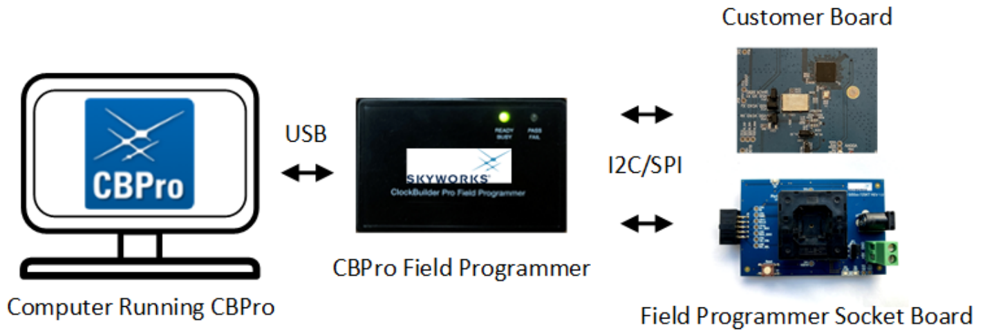
Figure 1.1. Example Hardware Configuration (Using QFN Socket Board or Customer PCB)
