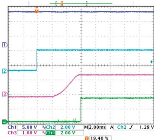
Start-up from ENABLE: 1 Vin, 1.5 Vout, 0 A Iout 2100 \mu F (external Cout: [10 x 22 \mu F]+[4 x 47 \mu F]). Trace 1 = Vin, Trace 2 = ENABLE, Trace 3 = Vout, Trace 4 =Power Good
