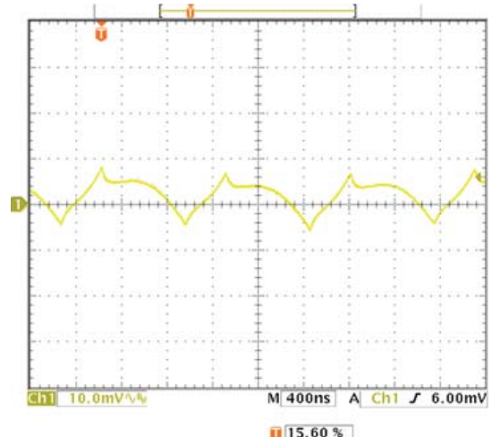
Output Ripple and Noise (V in = 12V, V out = 1.8V, I out = 50A, Cout = 10 \mu , T a = +25°C)
