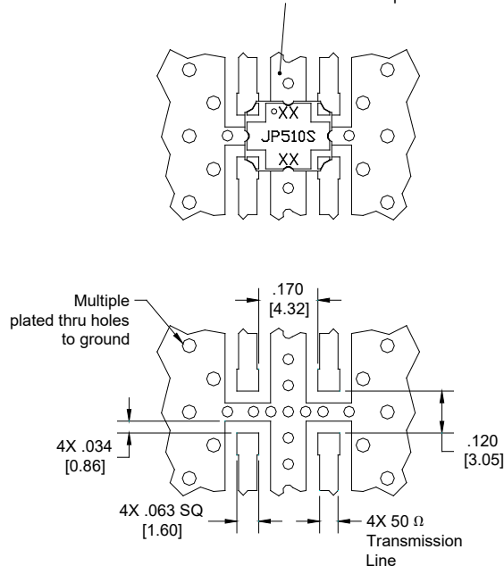
Dimensions are in Inches [Millimeters] JP510S Mounting Footprint
