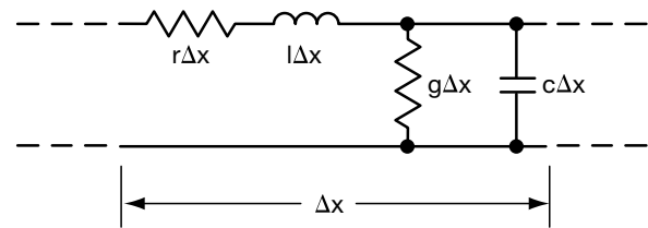
DISTRIBUTED PARAMETER MODEL OF A SECTION OF TRANSMISSION LINES:
