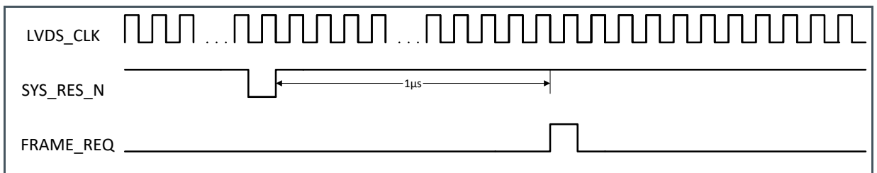
Figure 13: Reset Sequence
