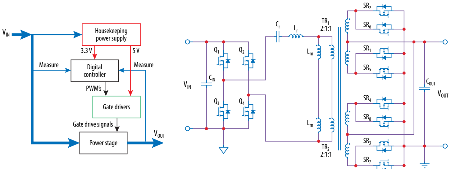
Figure 1: Simplified schematic diagram of the EPC9174 LLC Module
