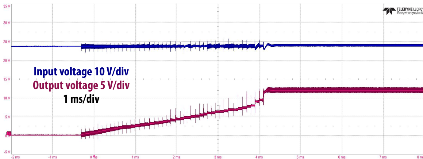
Figure 5: Startup waveform (larger time scale on top and zoomed in version on the bottom)
