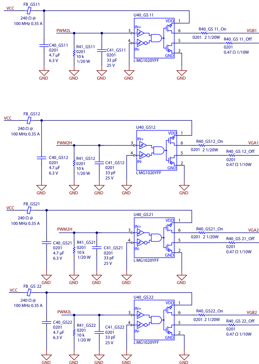
Secondary-side Gate Drivers
