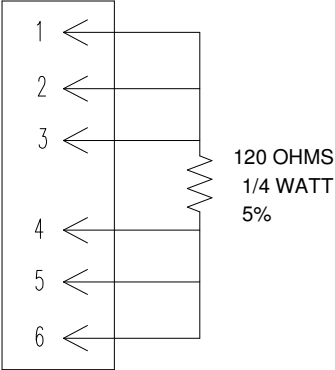
WIRING DIAGRAM
