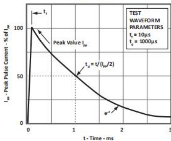
FIGURE 2 PULSE WAVEFORM
