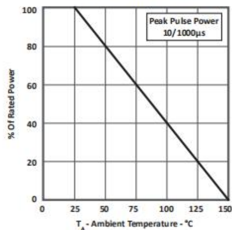
FIGURE 3 POWER DERATING CURVE
