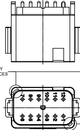
P/N AT04-12PD-BMXX KEY-D CONFIGURATION COLOR: BROWN
