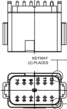
P/N AT04-12PB-BMXX KEY-B CONFIGURATION COLOR: BLACK
