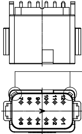
P/N AT04-12PA-BMXX KEY-A CONFIGURATION COLOR: GREY
