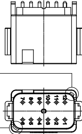
P/N AT04-12PC-BMXX KEY-C CONFIGURATION COLOR: GREEN
