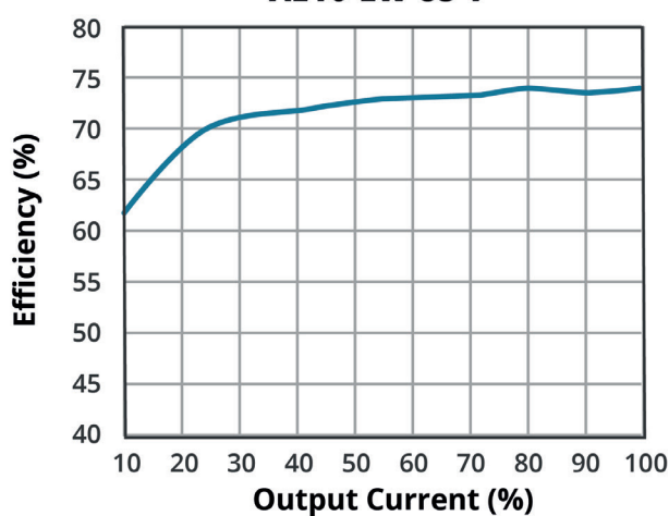
EFFICIENCY VS OUTPUT LOAD AE10-EW-S5-T
