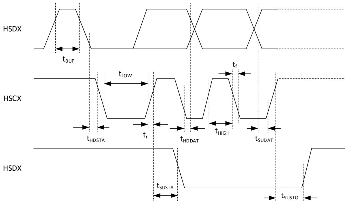
Figure 20: Host I2C interface timing
