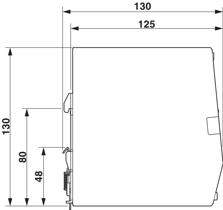
Dimensional drawing
