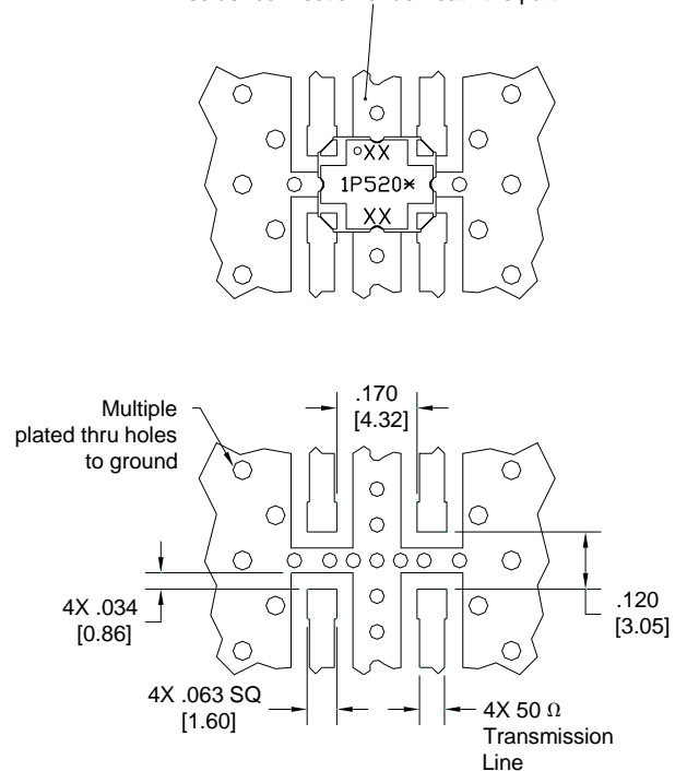
Dimensions are in Inches [Millimeters] 1P520* Mounting Footprint
