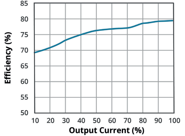
EFFICIENCY VS OUTPUT LOAD AE15-UW-S15
