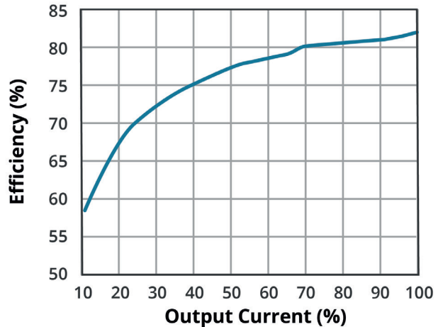
EFFICIENCY VS OUTPUT LOAD AE15-UW-S24
