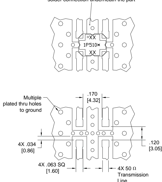
Dimensions are in Inches [Millimeters] 1P510* Mounting Footprint
