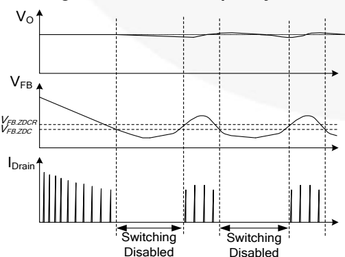
Figure 24. Burst-Mode Operation
