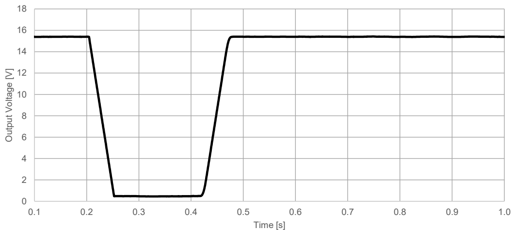
173011535 Short Circuit Protection, V_{IN} = 24V , V_{OUT} = 15V and I_{OUT} = 1A
