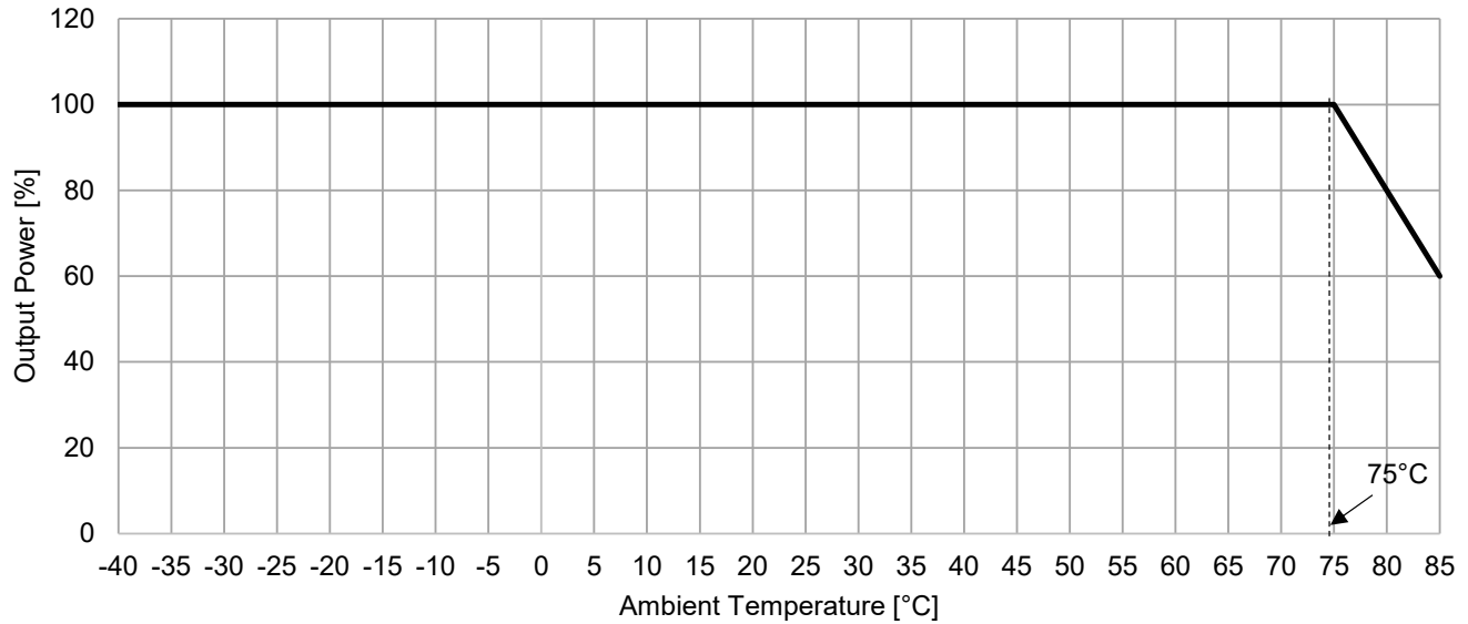
173010335, 173010535 Output Power Thermal Derating
