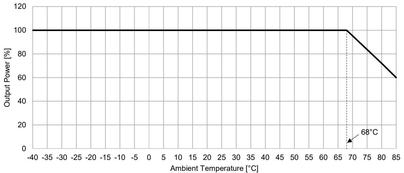
173011235, 173011535 Output Power Thermal Derating
