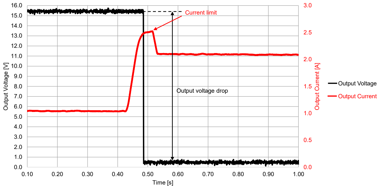
173011535 Overcurrent Protection, V_{IN} = 24V , T_A = 25^\circ C
