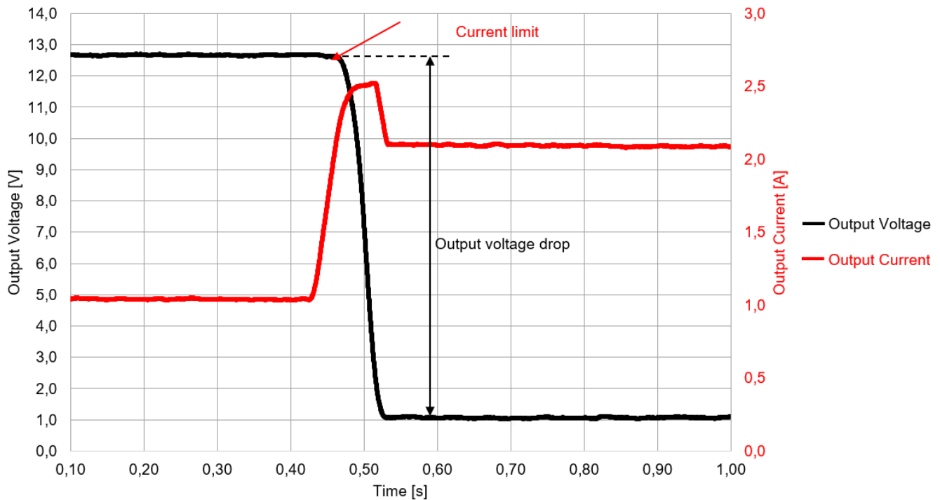
173011535 Overcurrent Protection, V_{IN} = 24V , T_A = 25^\circ C
