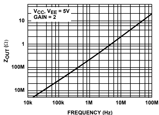
FIGURE 10. CLOSED LOOP OUTPUT IMPEDANCE vs FREQUENCY (6 LD SOT-23)
