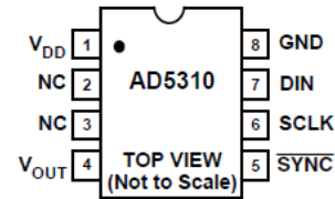
NC = NO CONNECT Figure 4. μSOIC
