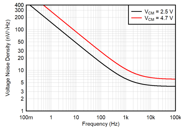
Figure 7-22. Voltage Noise vs Frequency
