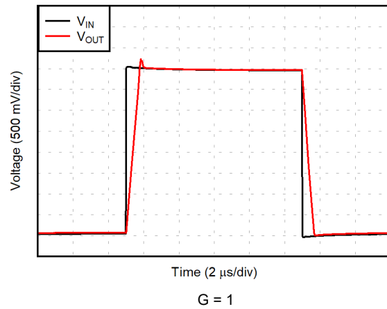
Figure 7-37. Large-Signal Step Response (4-V Step)
