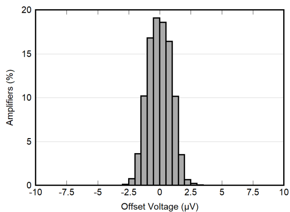
Figure 7-1. Offset Voltage Distribution
