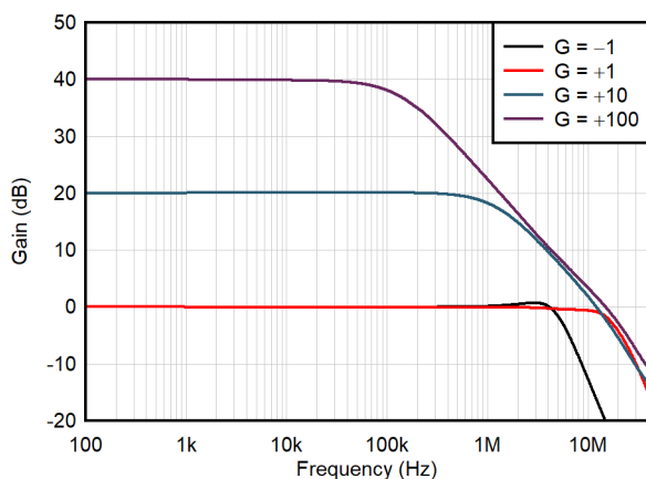
Figure 7-10. Closed-Loop Gain vs Frequency
