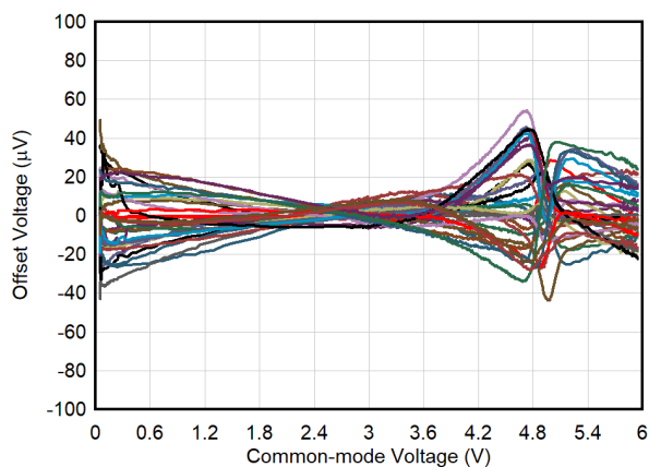
Figure 7-5. Offset Voltage vs Common-Mode Voltage
