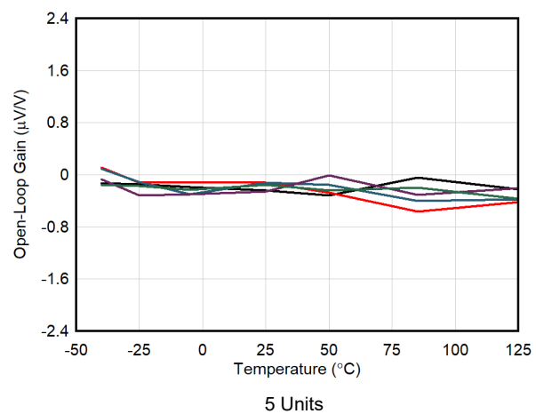
Figure 7-28. Open-Loop Gain vs Temperature
