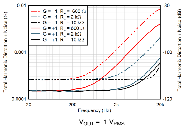
Figure 7-23. THD+N Ratio vs Frequency
