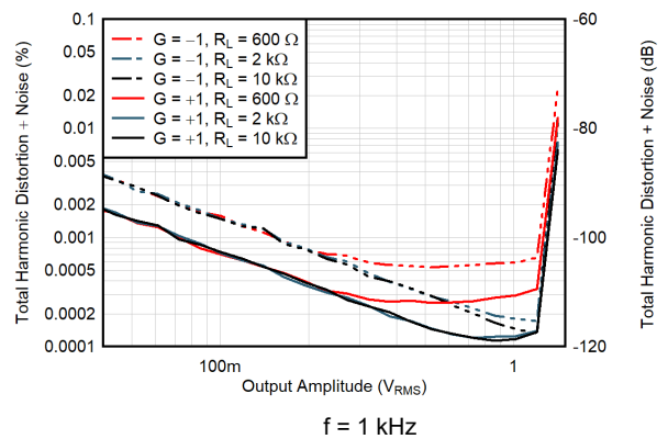
Figure 7-24. THD+N vs Output Amplitude
