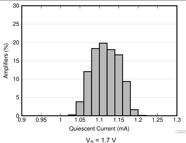
Figure 7-8. Quiescent Current Distribution
