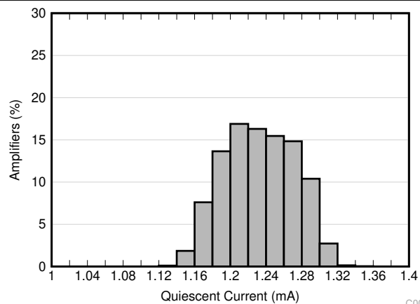
Figure 7-7. Quiescent Current Distribution
