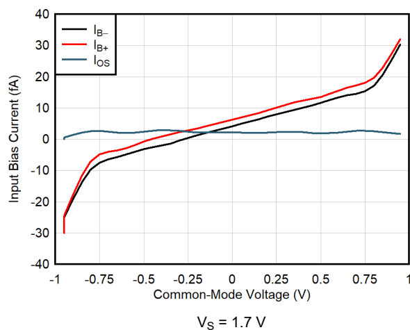
Figure 7-11. Input Bias Current vs Common-Mode Voltage
