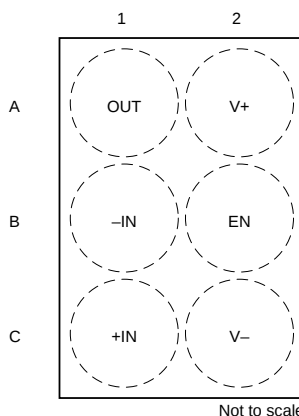
Figure 6-3. OPA392 YBJ Package (6-Pin DSBGA, Preview), Top View
