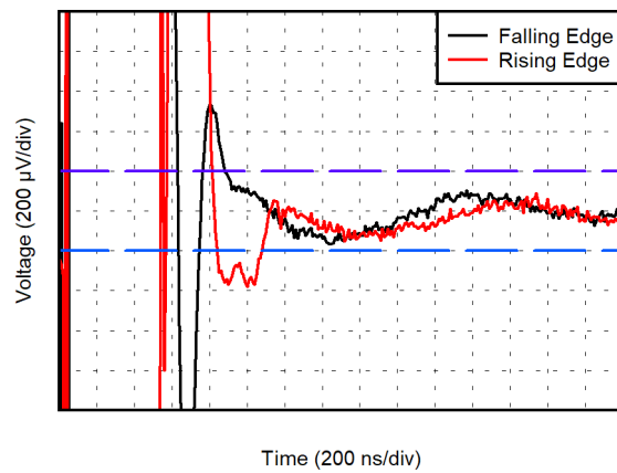
Figure 7-39. Settling Time
