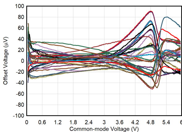
Figure 7-6. Offset Voltage vs Common-Mode Voltage
