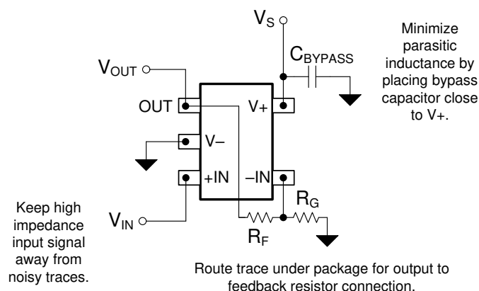
Figure 9-4. OPA392 Layout Example
