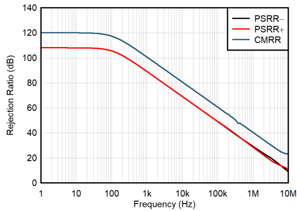
Figure 7-19. CMRR and PSRR vs Frequency
