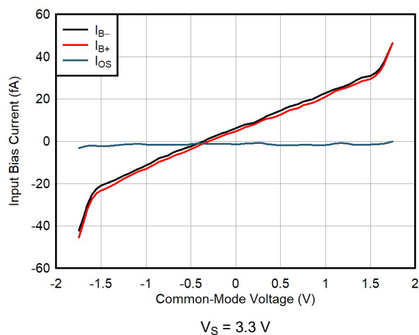
Figure 7-12. Input Bias Current vs Common-Mode Voltage
