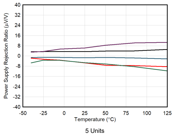
Figure 7-21. PSRR vs Temperature
