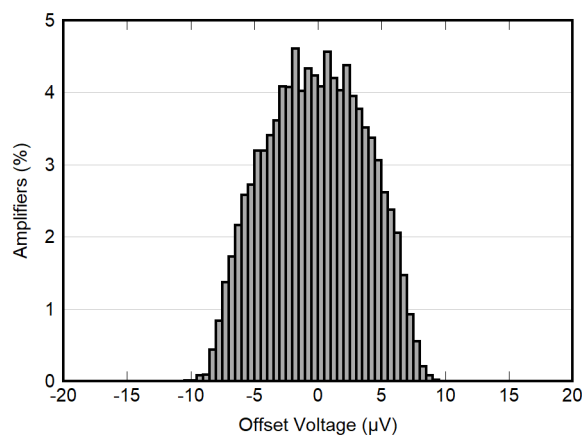
Figure 7-2. Offset Voltage Distribution
