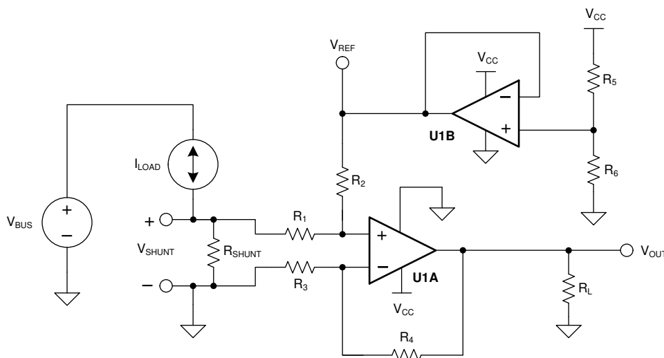
Figure 9-1. Bidirectional Current-Sensing Schematic
