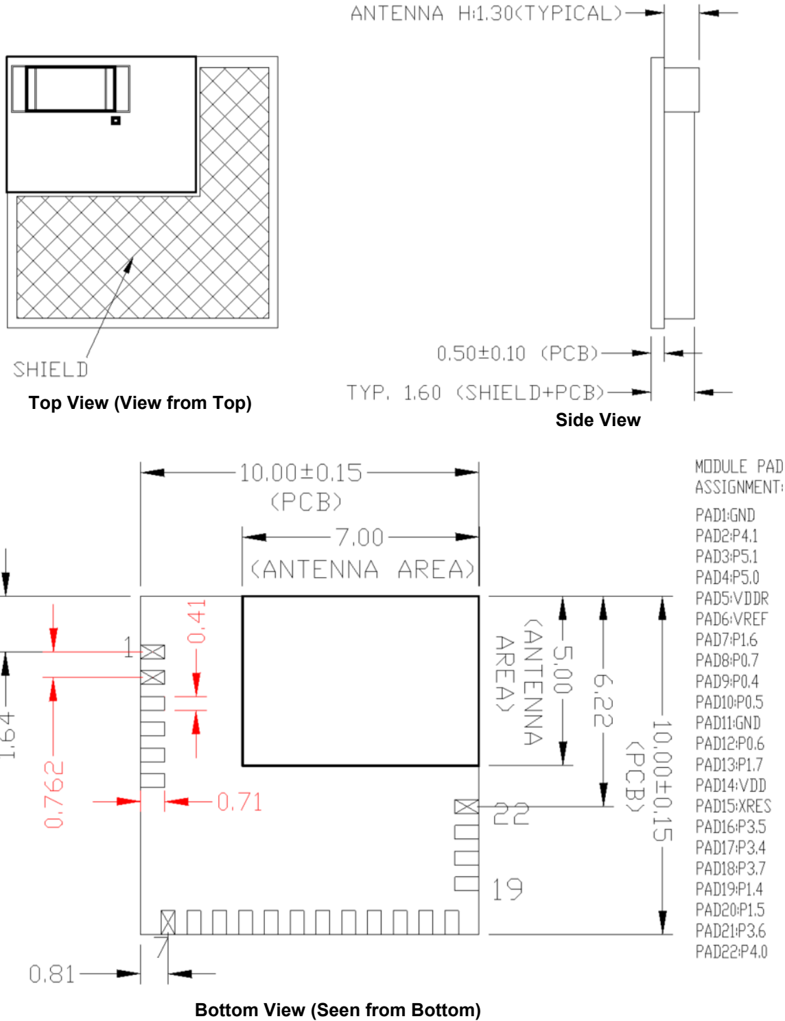
Figure 1. Module Mechanical Drawing
