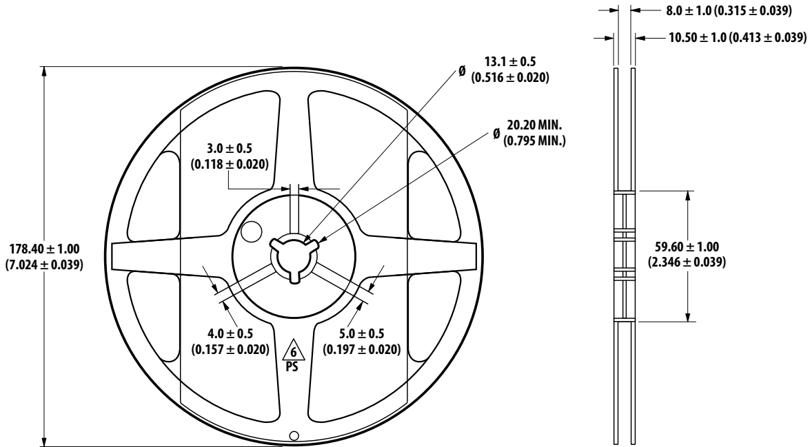
Figure 17: Reel Dimensions
