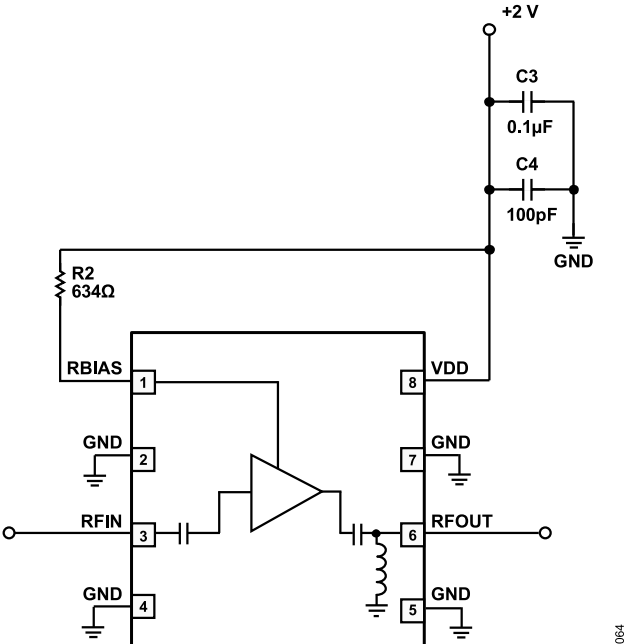
Figure 64. Typical Application Circuit
