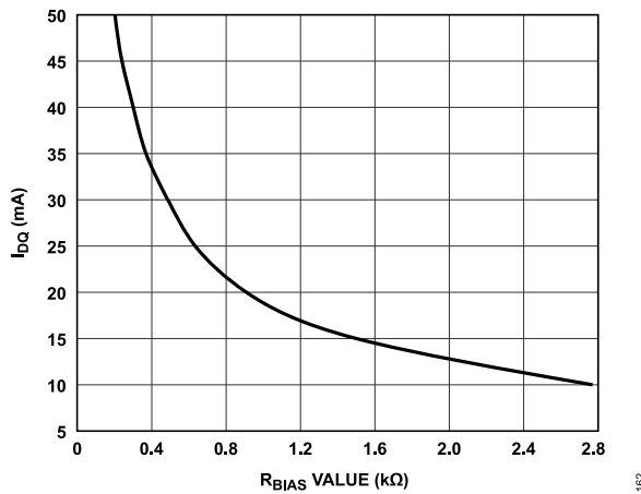
Figure 62. I_{DQ} vs. R_{BIAS} Value, V_{DD} = 2 V
