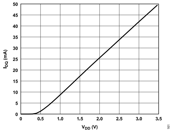
Figure 61. I_{DQ} vs. V_{DD} , R_{BIAS} = 634 \Omega
