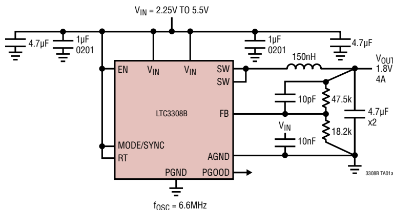
Small Solution Size, 6.6MHz, 1.8V 4A Step-Down Converter
