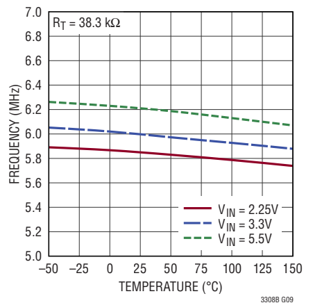
R_T Switching Frequency
