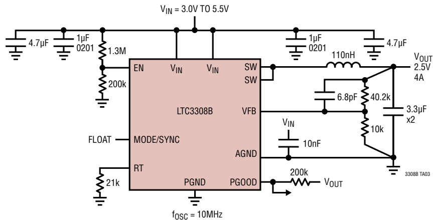
Ultralow Profile, V_{IN} UVLO 3.0V, 10MHz, 2.5V, 4A, Forced Continuous Mode
