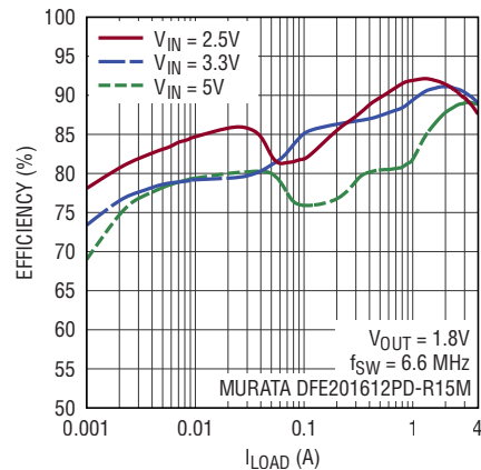
Efficiency in Burst Mode Operation
