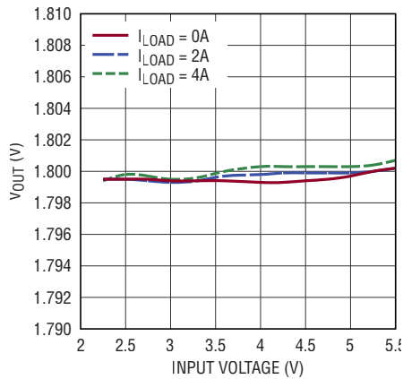
V_{OUT} Load Regulation in V_{OUT} = 1.8V Application
