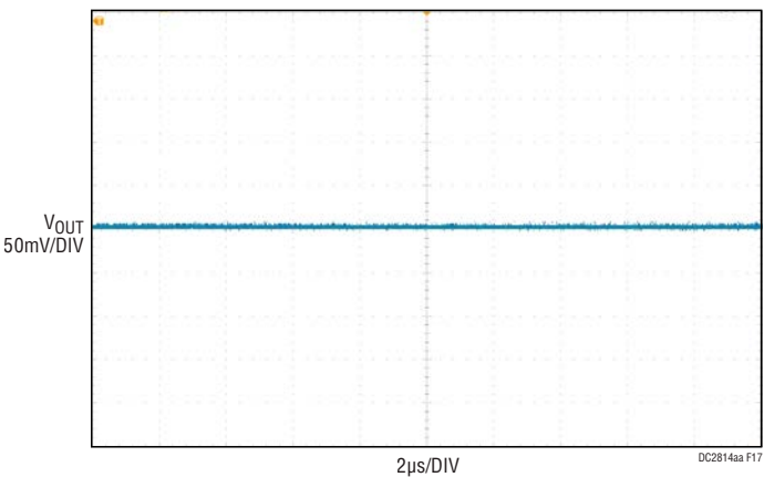
Figure 17. DC2814A-A Output Voltage Ripple at 12V IN (Pass-Thru), 12V OUT , 3A Load Current
