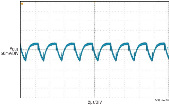
Figure 11. DC2814A-A Output Voltage Ripple at 6V IN (Boost), 8V OUT , 3A Load Current
