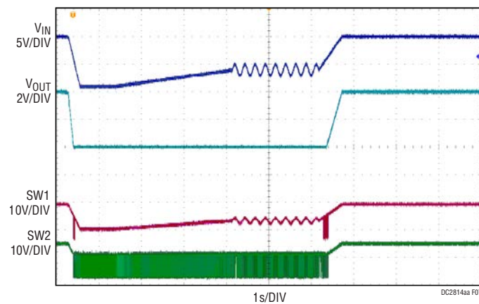
Figure 7. ISO16750 4.6.3, Starting Profile ( I_{OUT} = 1.5A )
