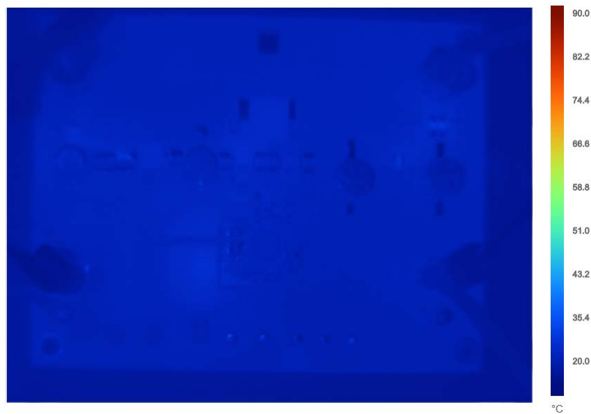
Figure 15. DC2814A-A Thermal Performance at 12V IN (Pass-Thru), 12V OUT , 3A Load Current
