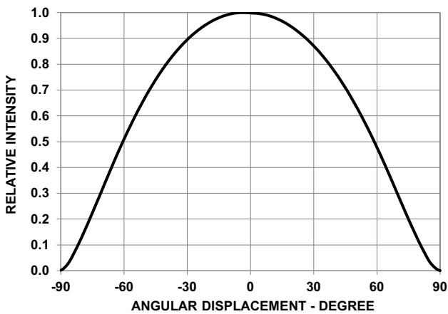
Figure 6: Radiation Pattern
