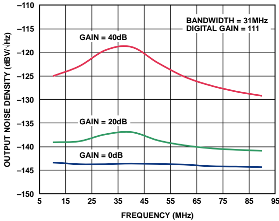
Figure 35. Output Noise Density vs. Frequency (Bandwidth Setting = 31 MHz, Digital Gain = 111)
