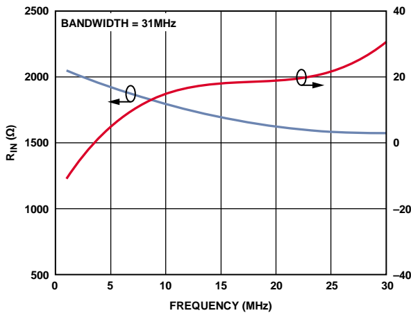
Figure 37. Input Impedance vs. Frequency (Bandwidth Setting = 31 MHz)
