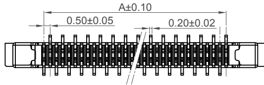
Right Footprint Version (Standard)
