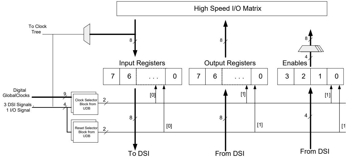
Figure 6. Port Interface
