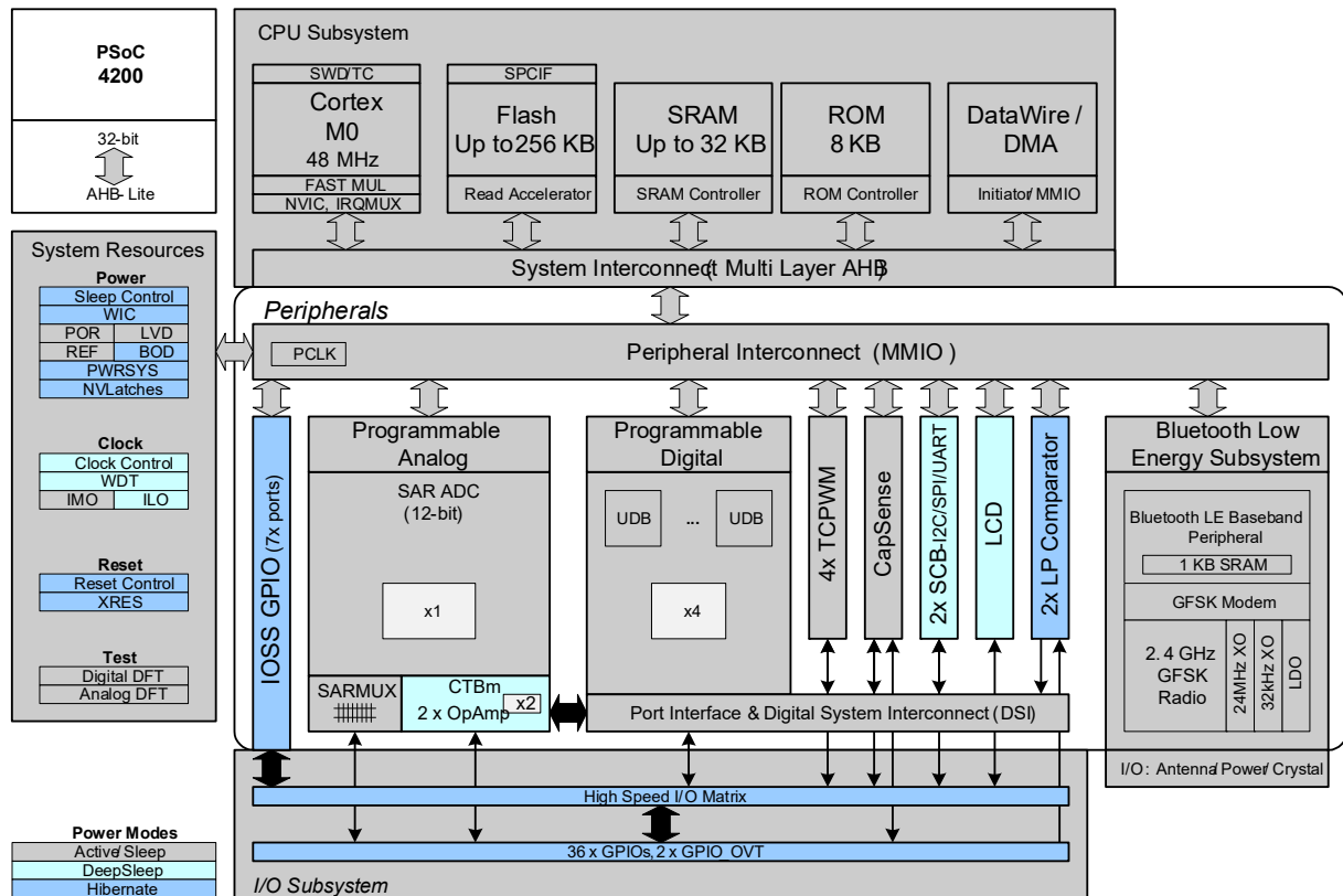
Figure 2 Block Diagram
