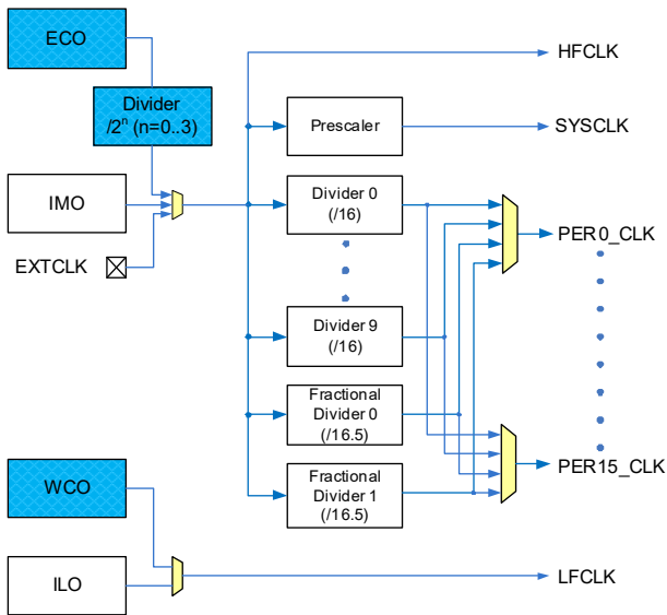
Figure 3 PSoC™ 4 CY8C42xx-BL MCU with AIROC™ Bluetooth® LE MCU Clocking Architecture
