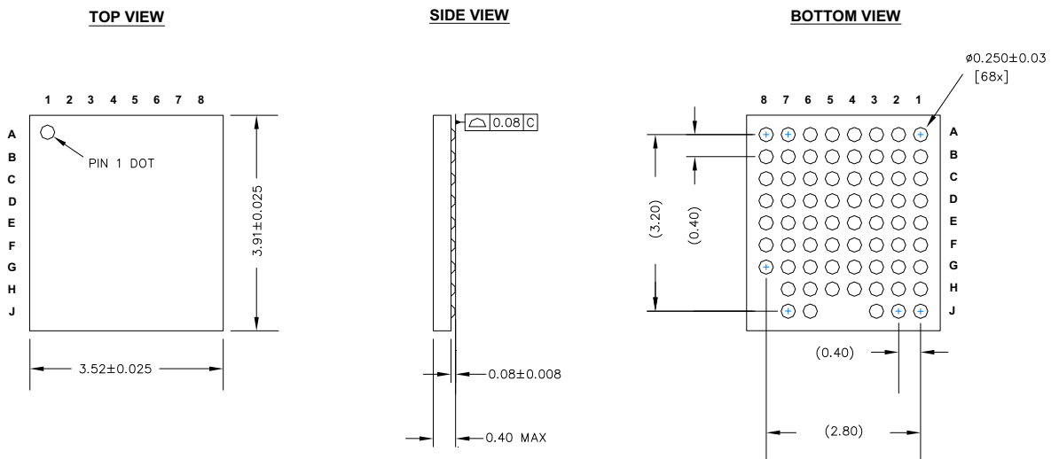
Figure 1168-Ball Thin WLCSP
