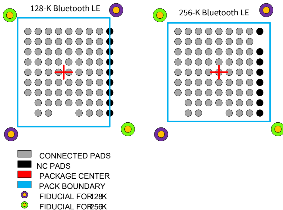
Figure 9 128KB and 256 KB Flash CSP Packages
