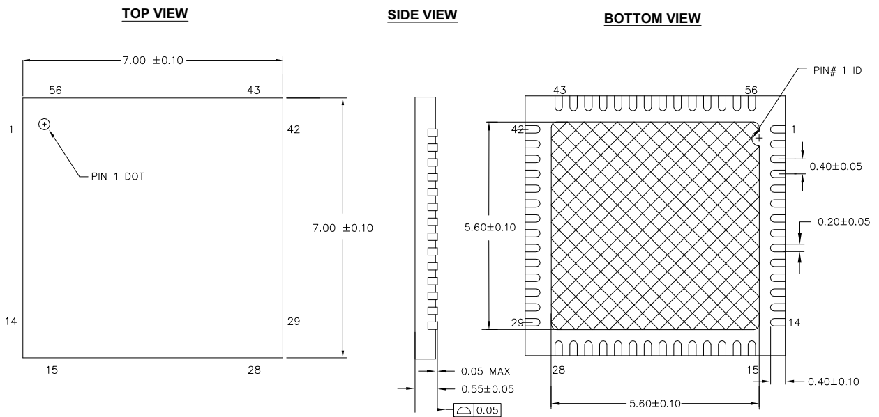
Figure 856-Pin QFN 7 × 7 × 0.6 mm
