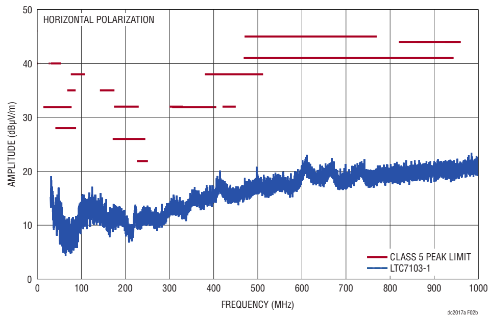
Figure 2. EMI Performance in CISPR 25 Radiated Emission Test (48V IN from +VIN_EMI Turret Pin, 5V OUT /2A, f SW = 400kHz)
