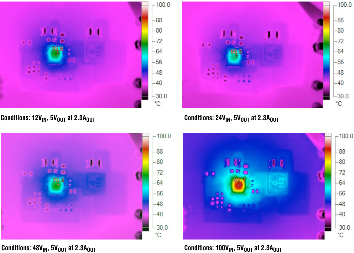
Figure 7. Thermal Plots ( T_A = 25^{\circ}\text{C} , without Forced Air)
