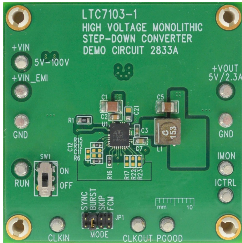
Figure 8. Board Photo
