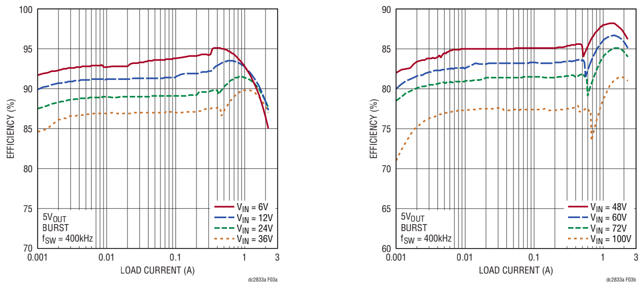
Figure 3. Efficiency at Various Input Voltages (Conditions: Burst Mode Operation)
