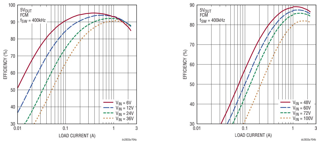
Figure 4. Efficiency at Various Input Voltages (Conditions: Forced Continuous Mode)
