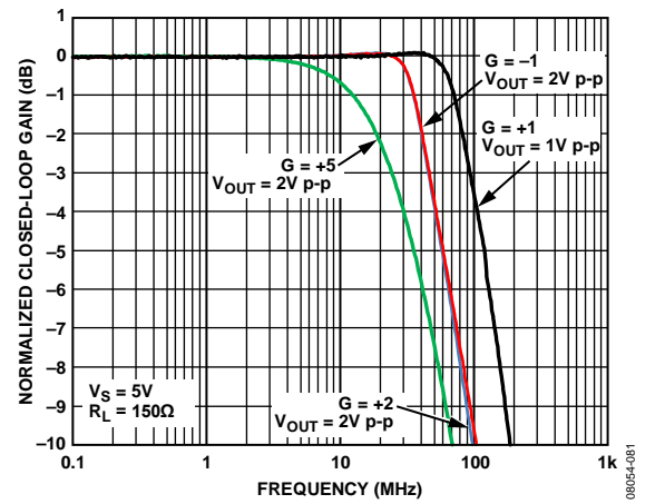
Figure 18. Large-Signal Frequency Response vs. Gain, V_S = 5V , ADA4891-3/ADA4891-4
