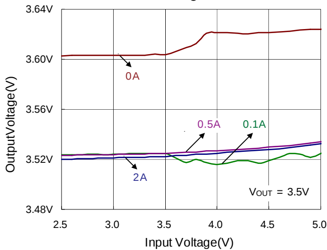
Line Regulation
