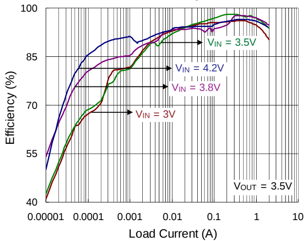
Efficiency
