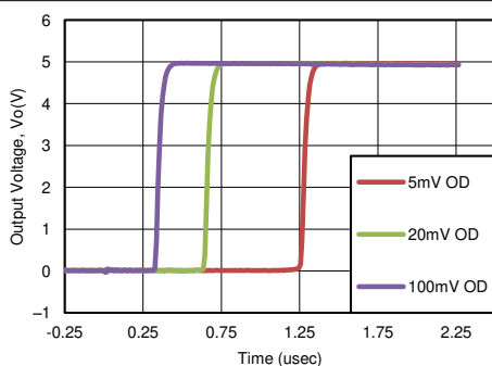
Figure 8-2. Response Time for Various Overdrives (Positive Transition)
