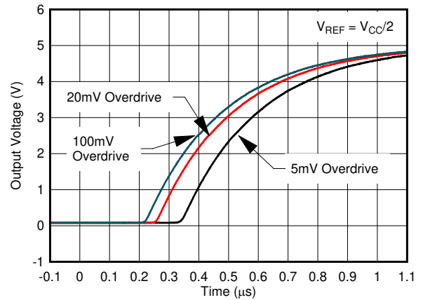
Figure 6-37. Response Time for Various Overdrives, Low-to-High Transition
