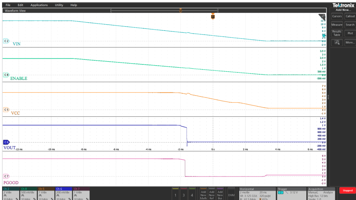
Figure 21 Shutdown with Enable de-assertion at 12A load (Ch2:PV IN , Ch5:V CC , Ch6: V OUT , Ch7: PGood, Ch8: Enable)
