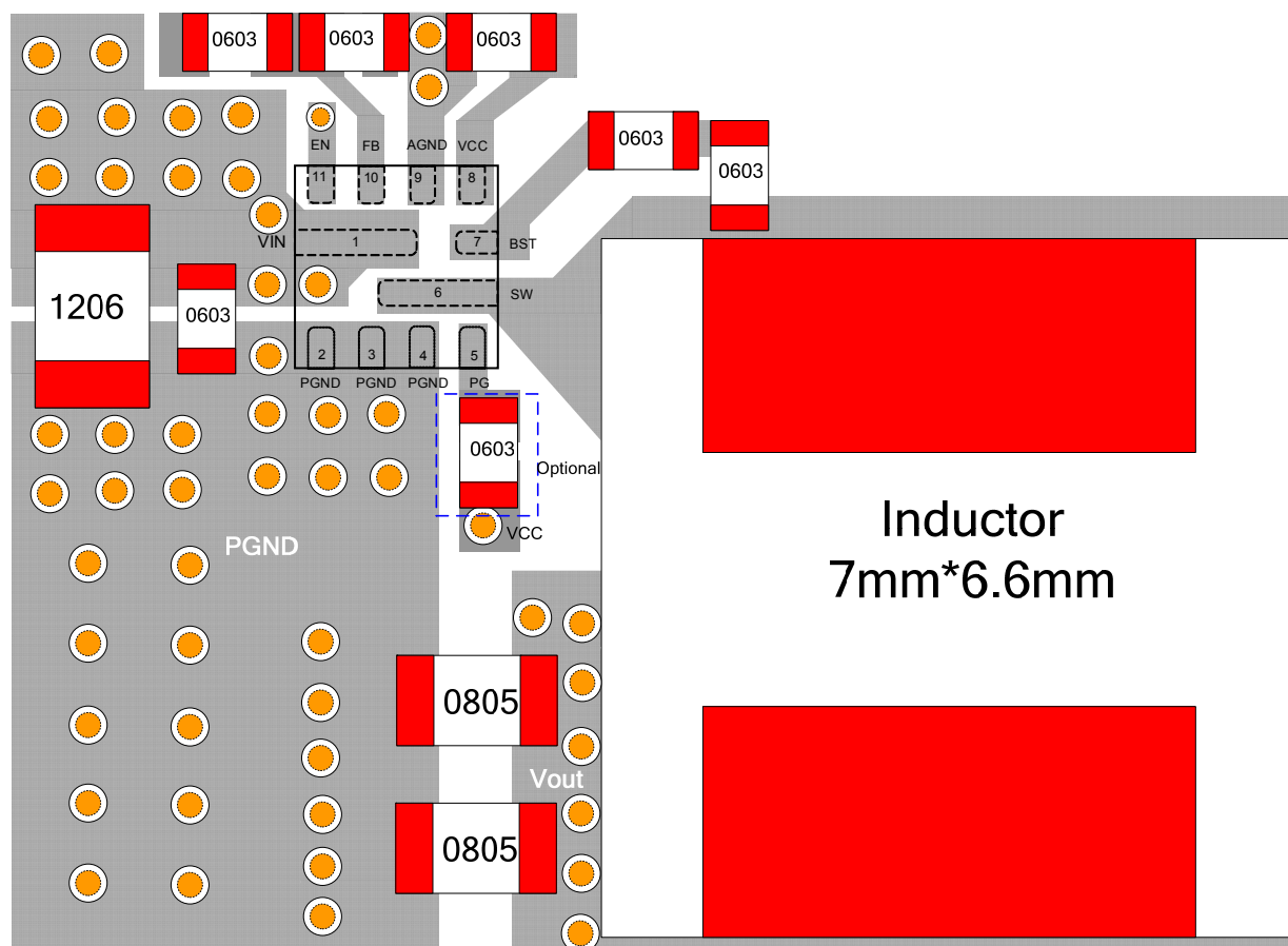
Figure 10: Recommended Layout
